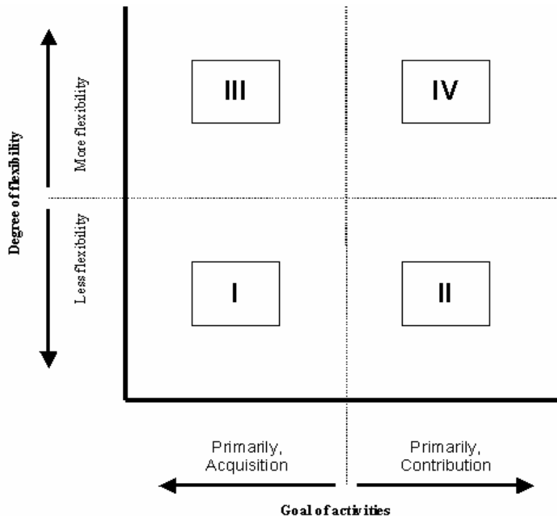
Figure 1: Flexibility-activity framework
